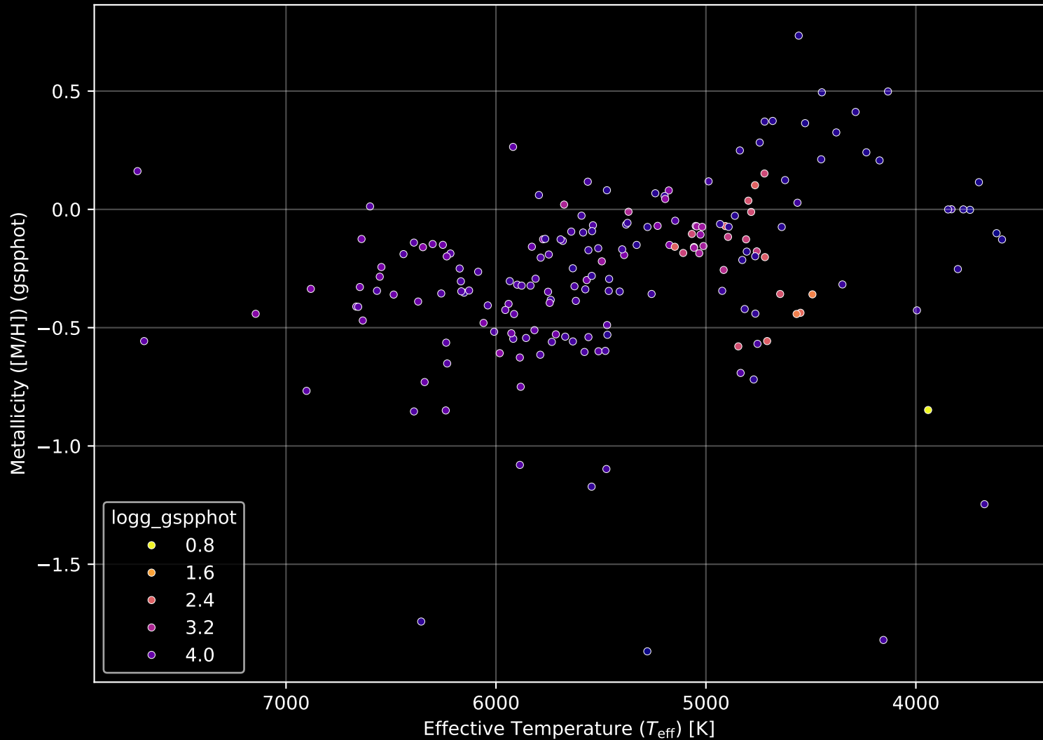
APOGEE DR17 Field: [133-48_MGA] Stellar Population Parameters (n= 185)
