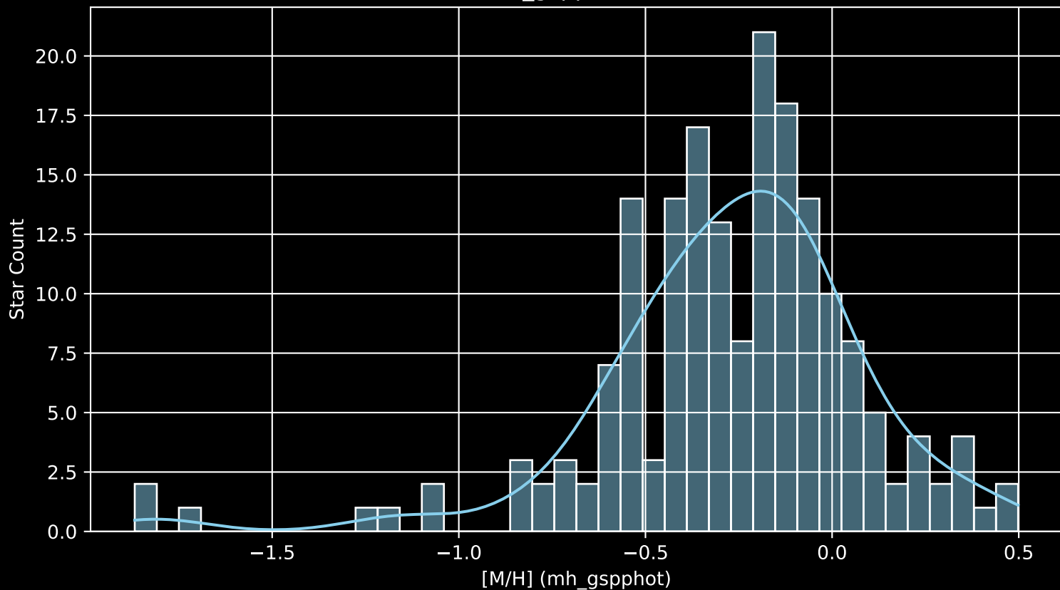
APOGEE DR17 Field: [133-48_MGA [M/H] (mh_gspphot) (n= 184)
