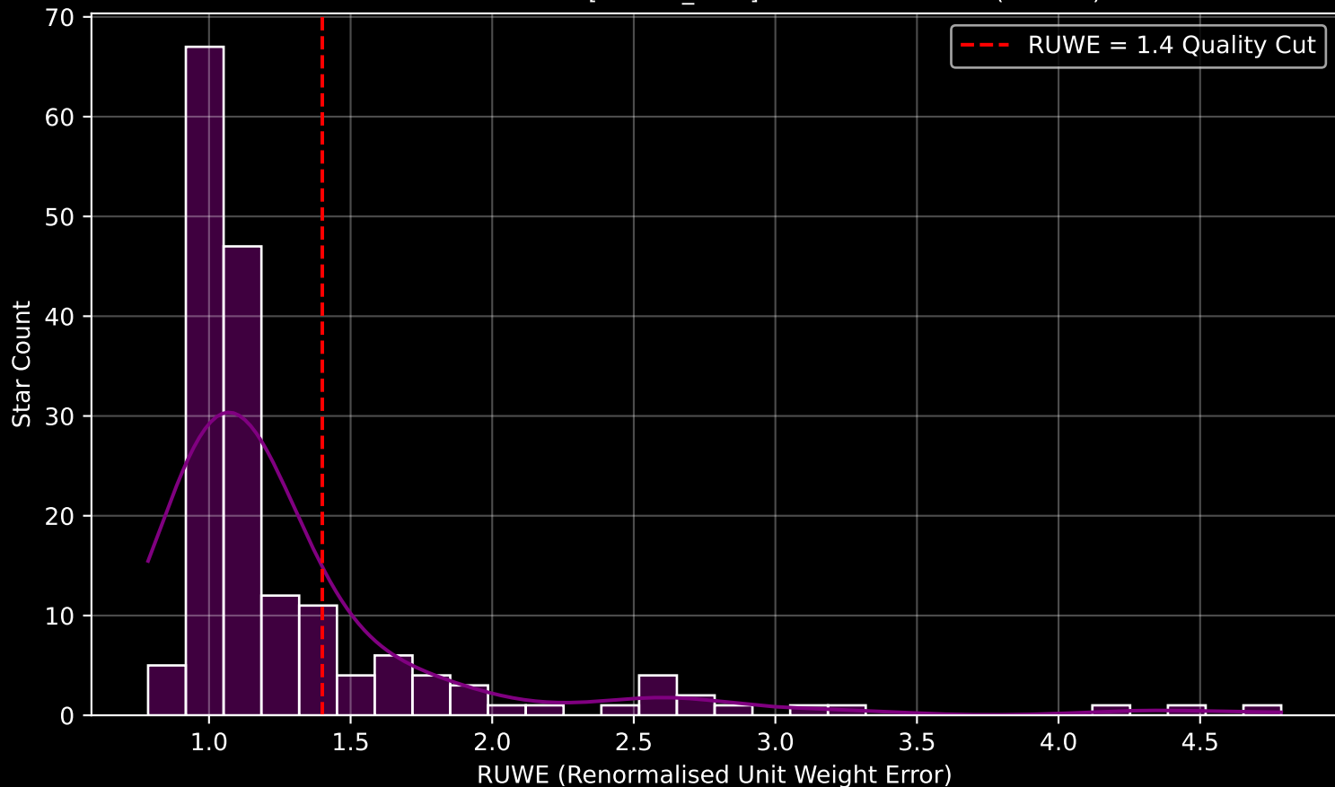
GAPOGEE DR17 Field [133-48_MGA] RUWE Distribution (n= 174)
