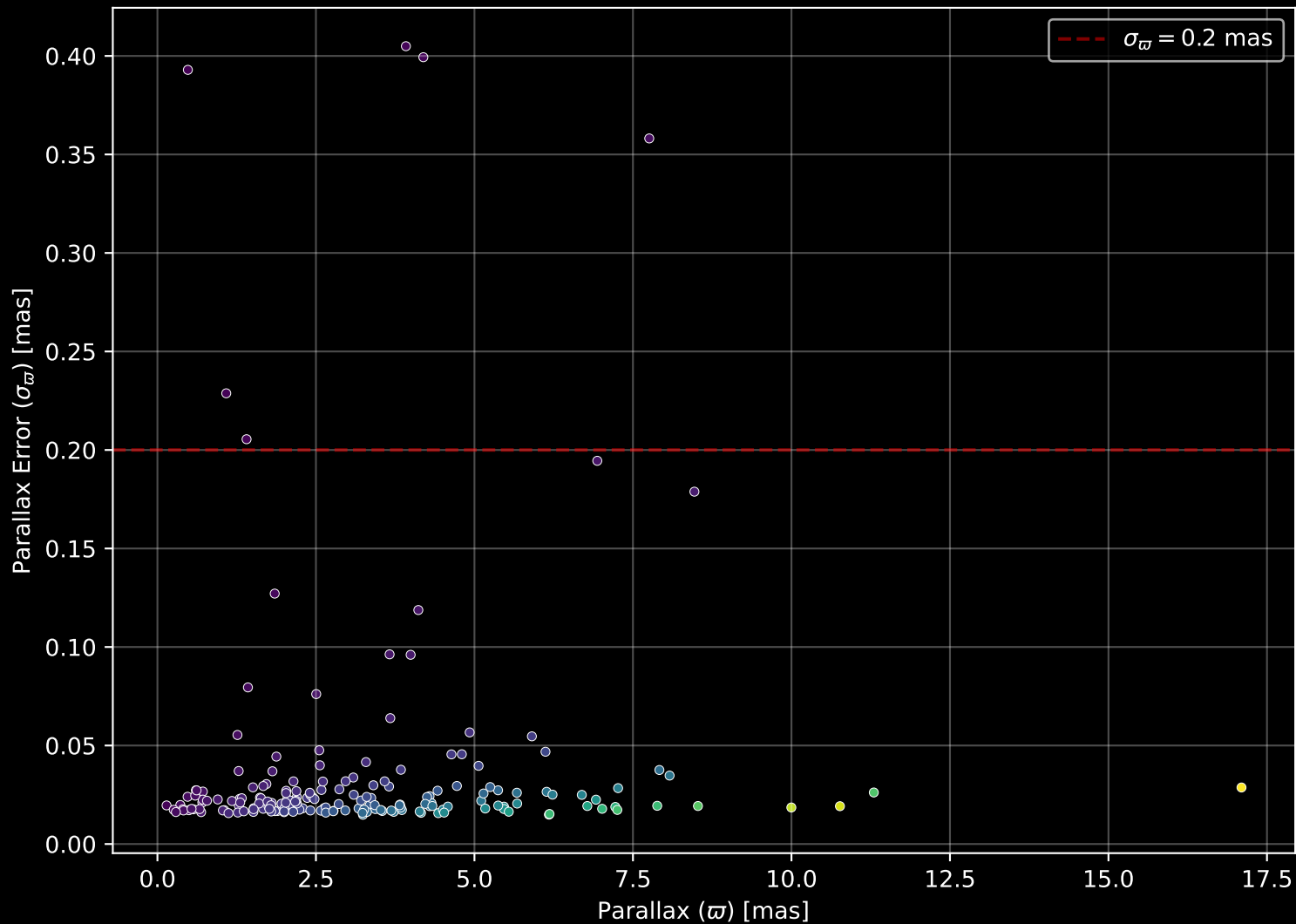
APOGEE DR17 Field: [133-48_MGA] Parallax Quality (n= 185)
