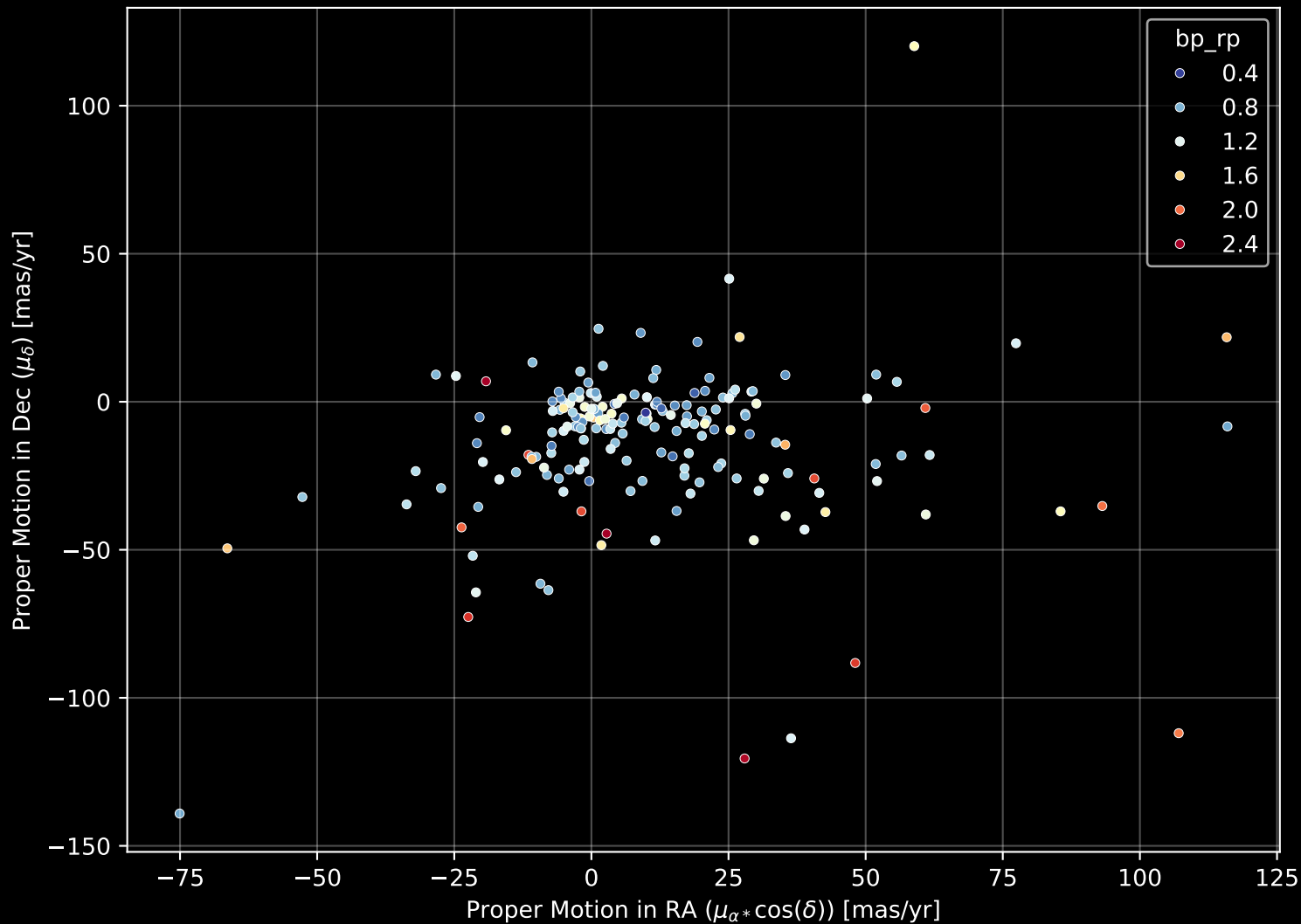
APOGEE DR17 Field: [133-48_MGA] Proper Motion Diagram (n= 185)
