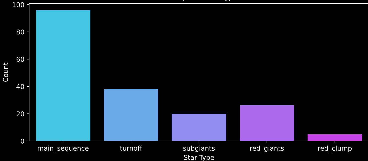
APOGEE DR17 Field: [133-48_MGA] Count plot of Star Type
